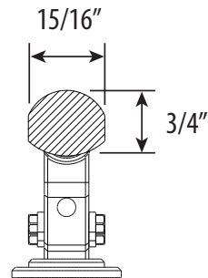
END VIEWS
